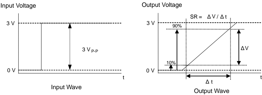
Figure 73. Slew Rate Input and Output Wave
