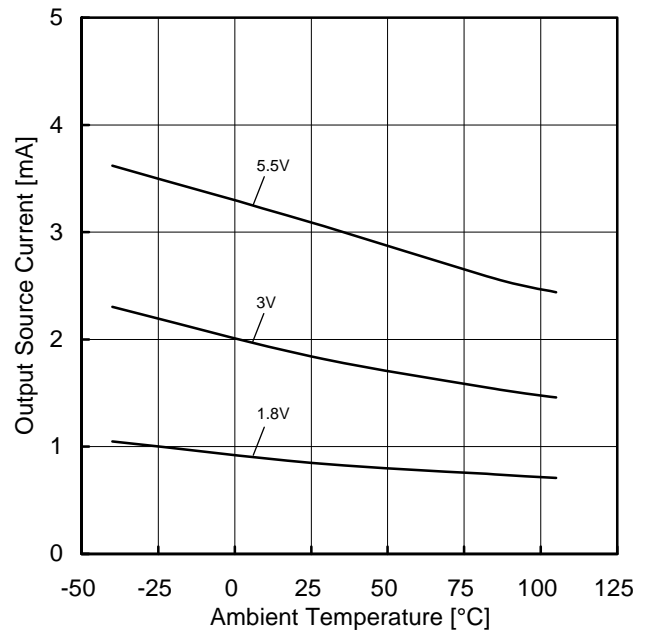
Figure 32. Output Source Current vs Ambient Temperature (OUT=VDD-0.4V)
