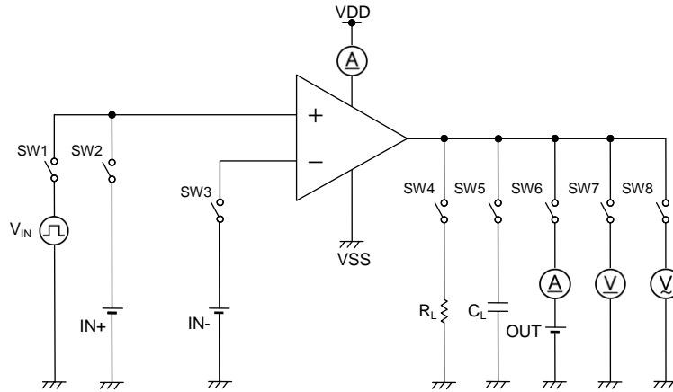
Figure 46. Test Circuit 2 (each channel)
