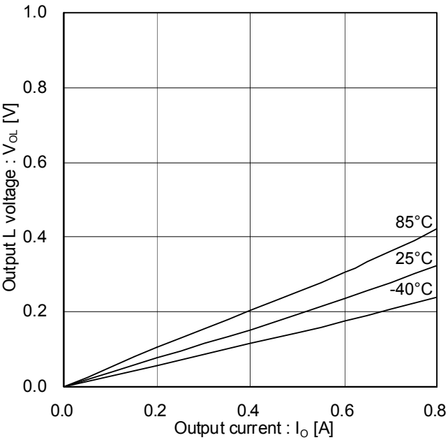
Figure 10. Output L Voltage (Temperature Characteristics)
