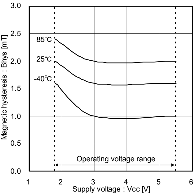
Figure 7. Magnetic hysteresis
