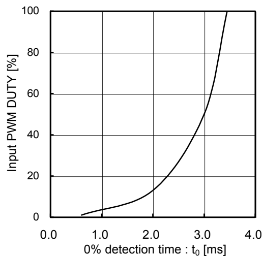
Figure 28. Characteristic curve of 0% detection time and input PWM duty at 25kHz
