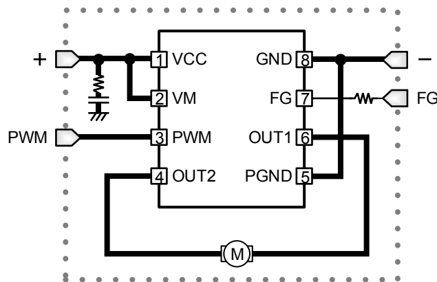
Figure 1. Application circuit
