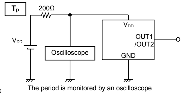
Figure 2. T p Measurement Circuit
