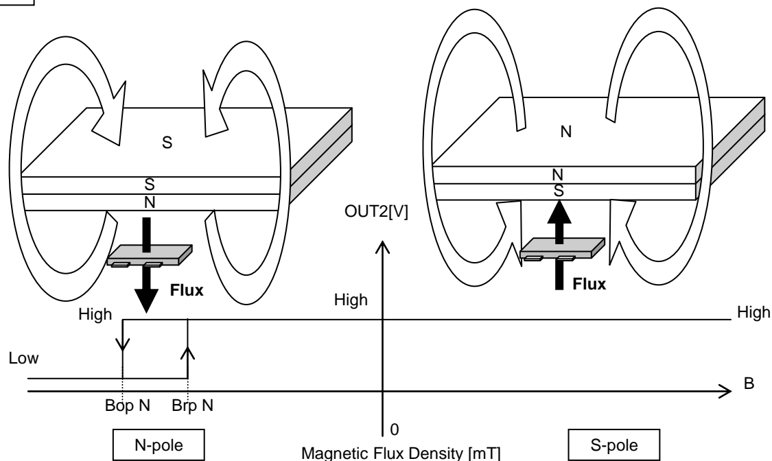
Figure 16. N-pole Detection
