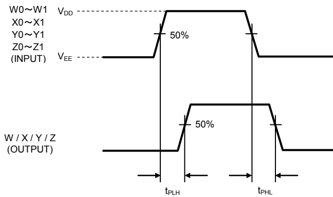
Figure 1. Propagation Delay Time (IN→OUT) (t PLH , t PHL )
