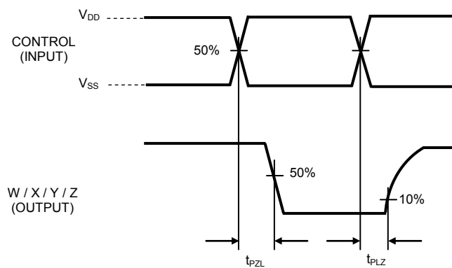
Figure 5. Propagation Delay Time (CONTROL→OUT) (t PZL , t PLZ )
