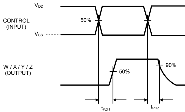
Figure 3. Propagation Delay Time (CONTROL→OUT) (t PLH , t PHL )
