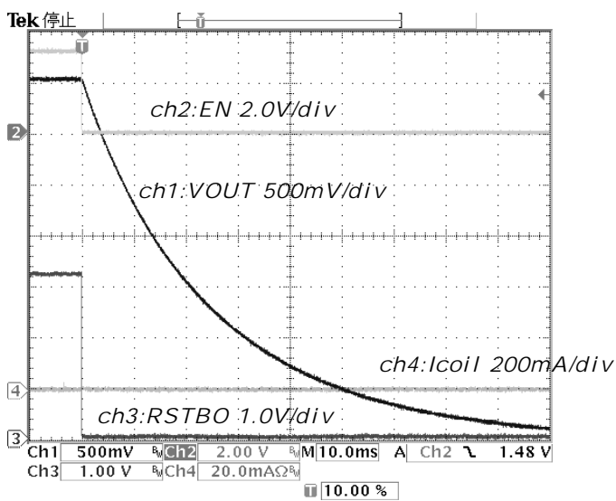
Figure 31. FALL [EN : ON=>OFF] PFM VIN=3.3V Io=0mA
