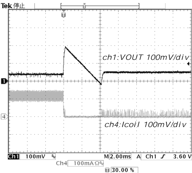
Figure 45. Io change PFM 100mA=>1mA VIN=3.3V
