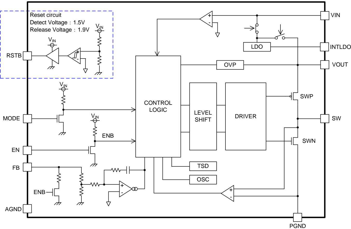
Figure 4. Circuit Block
