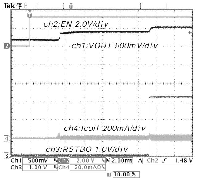
Figure 24. RISE [EN : OFF=>ON] PWM VIN=3.2V Io=0mA
