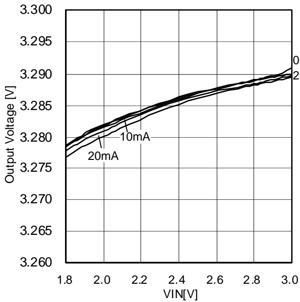
Figure 14. Line-Regulation[Ta=-30°C]
