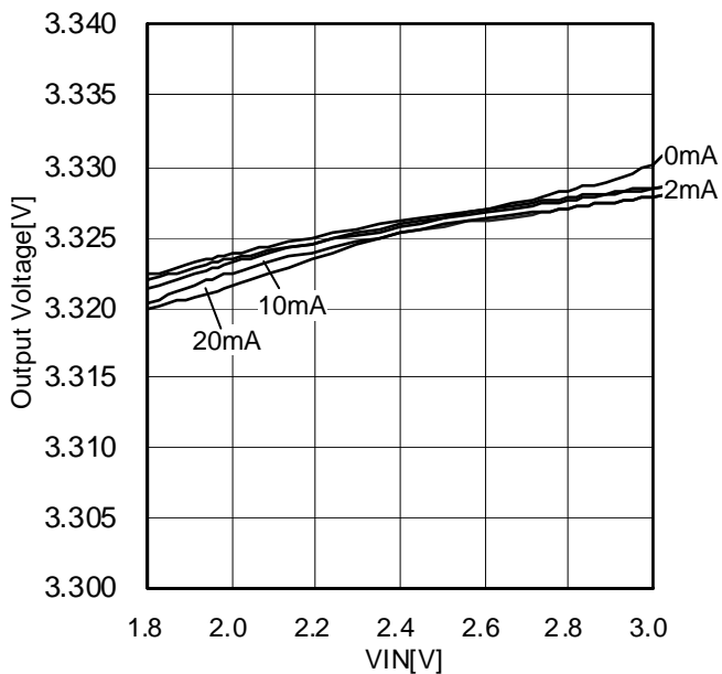
Figure 16. Line-Regulation[Ta=-85°C]
