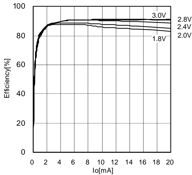
Figure 9. Efficiency[Ta=25°C]
