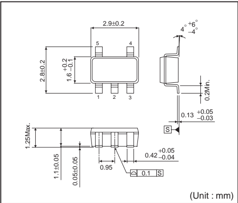
Figure 4. Package
