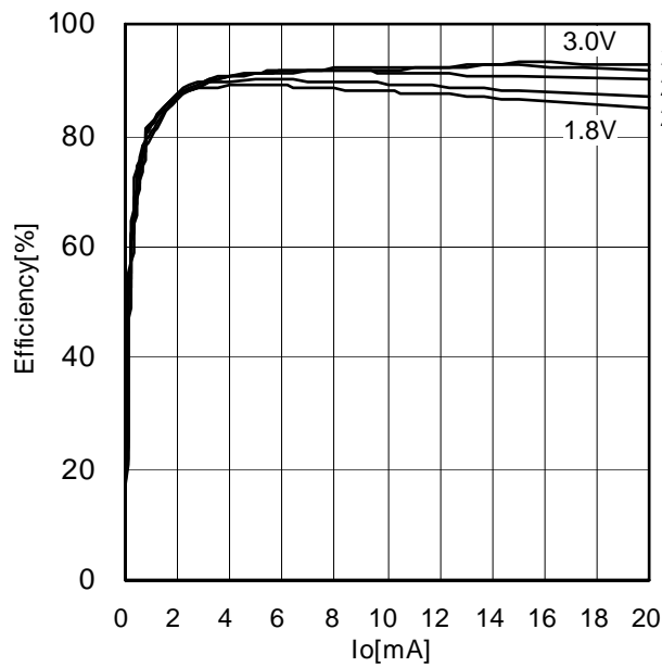
Figure 8. Efficiency[Ta=-30°C]
