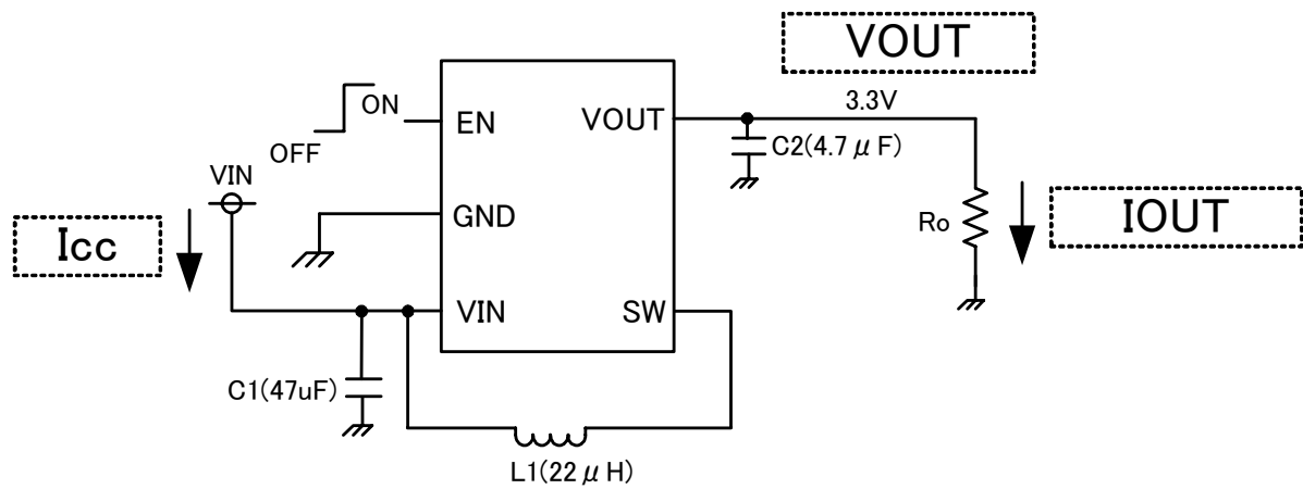
Figure 17. Measure circuit
