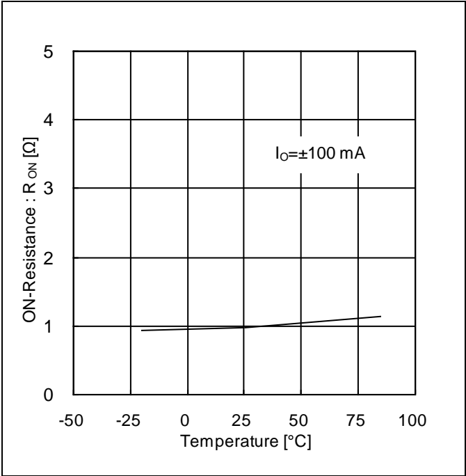
Figure 8. ON-Resistance vs Temperature (Current Driver Block)
