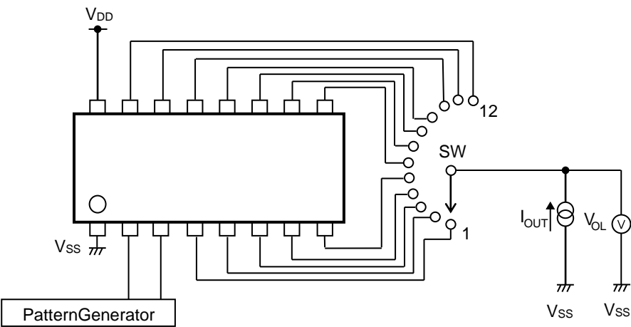
Figure 3. Test Circuit of Output L Voltage
