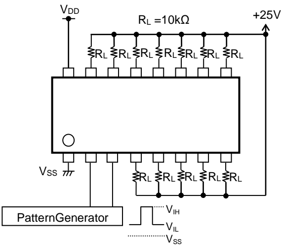
Figure 2. Test Circuit of Input H/L Voltage
