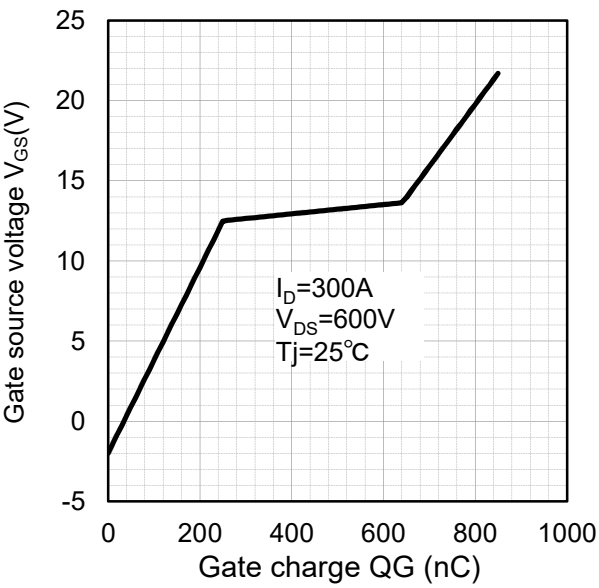
Fig.25 Gate charge characteristic (TYP)
