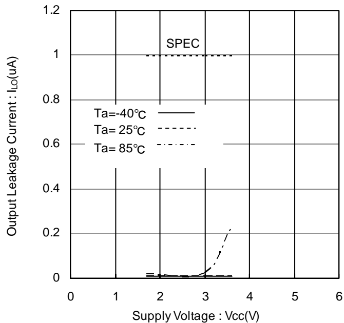
Figure 8. Output Leakage Current vs Supply Voltage (SDA)
