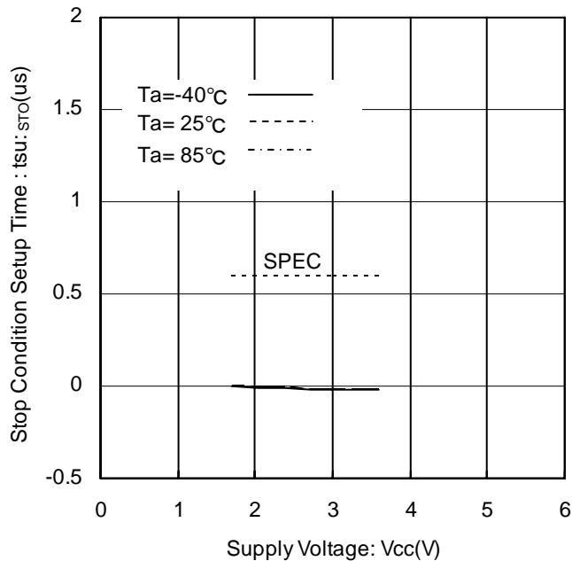
Figure 21. Stop Condition Setup Time vs Supply Voltage
