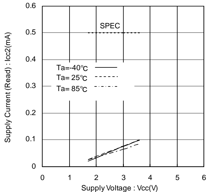
Figure 10. Supply Current (Read) vs Supply Voltage ( f_{SCL}=400kHz )
