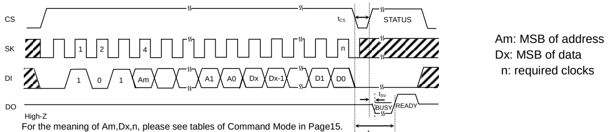
Figure 36. Write Cycle
