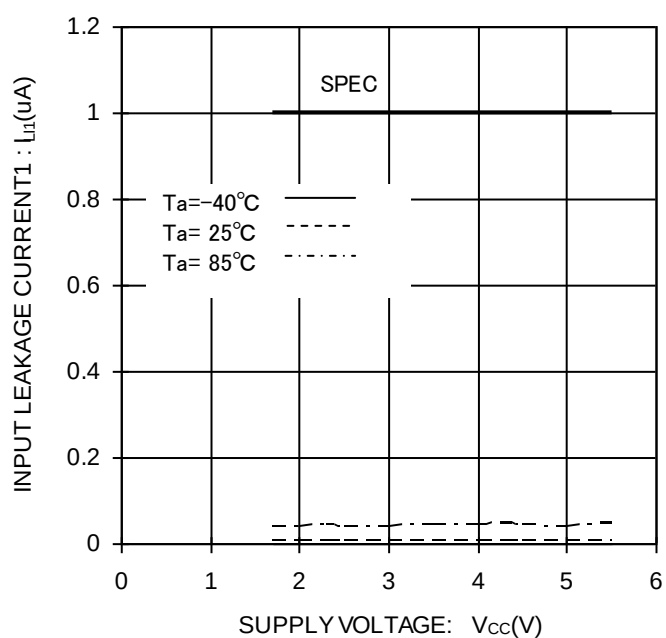
Figure 11. Input Leakage Current (SK) vs Supply Voltage
