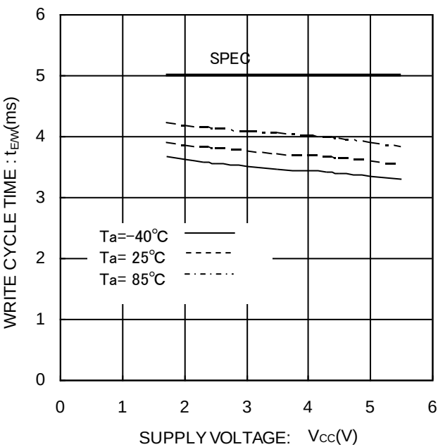
Figure 33. Write Cycle Time vs Supply Voltage
