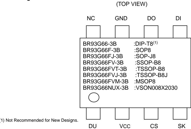
Figure 3. Pin Configuration
