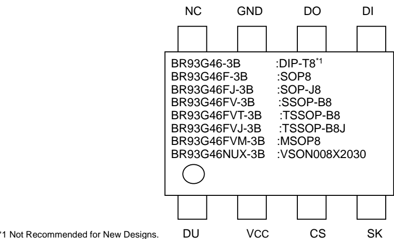
Figure 3. Pin Configuration
