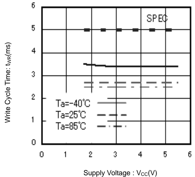
Figure 25. Write Cycle Time vs Supply Voltage
