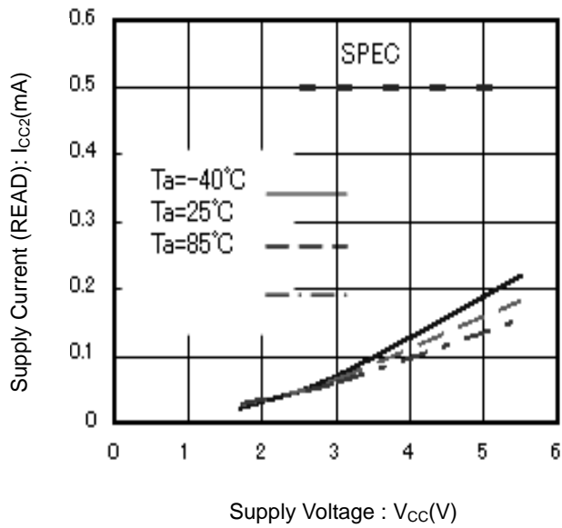
Figure 10. Supply Current (READ) vs Supply Voltage ( f_{SCL}=400kHz )
