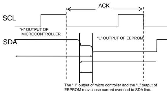
Figure 47. Input/Output Collision Timing
