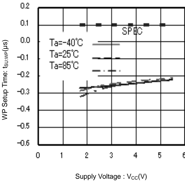
Figure 31. WP Setup Time vs Supply Voltage
