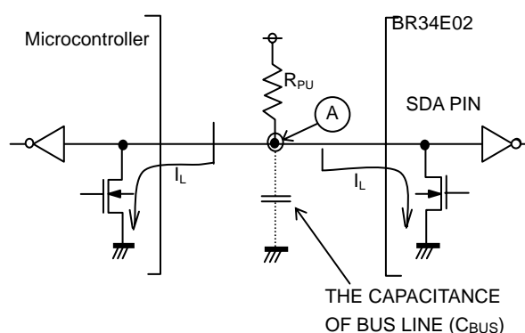
Figure 45. I/O Circuit
