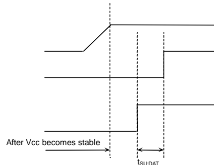
Figure 55. SCL="L" and SDA="L"
