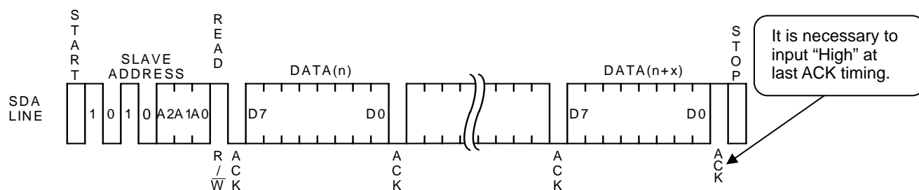
Figure 37. Sequential Read Cycle Timing (With Current Read)
