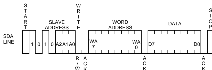
Figure 33. Byte Write Cycle Timing
