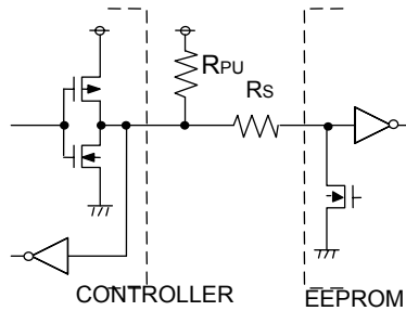
Figure 44. I/O Circuit
