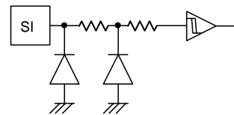
Figure 48. SI input equivalent circuit
