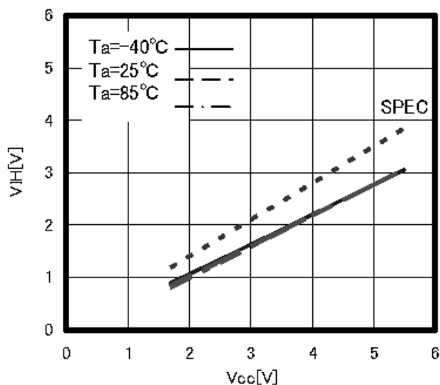
Figure 4. "H" Input Voltage V_{IH} (CSB, SCK, SI, HOLDB, \overline{\text{WP}} )
