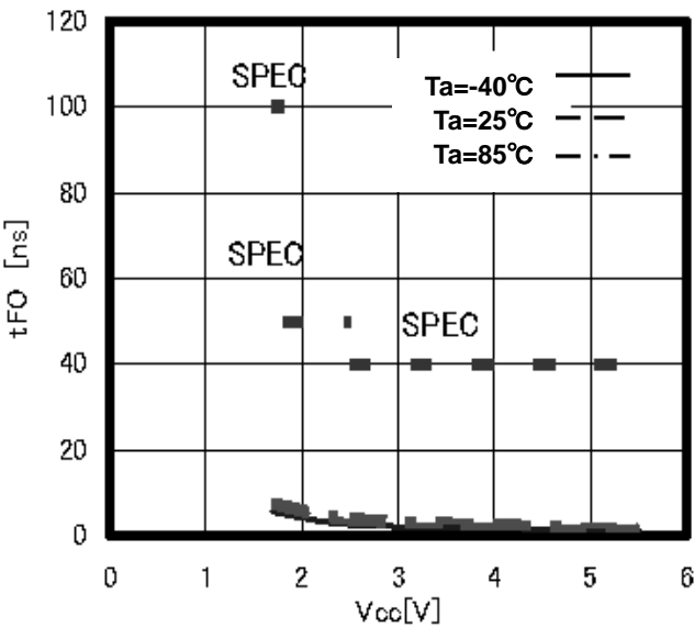
Figure 28. Output fall time tFO
