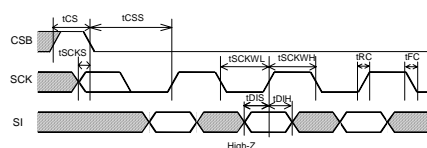
Figure 1. Input timing
