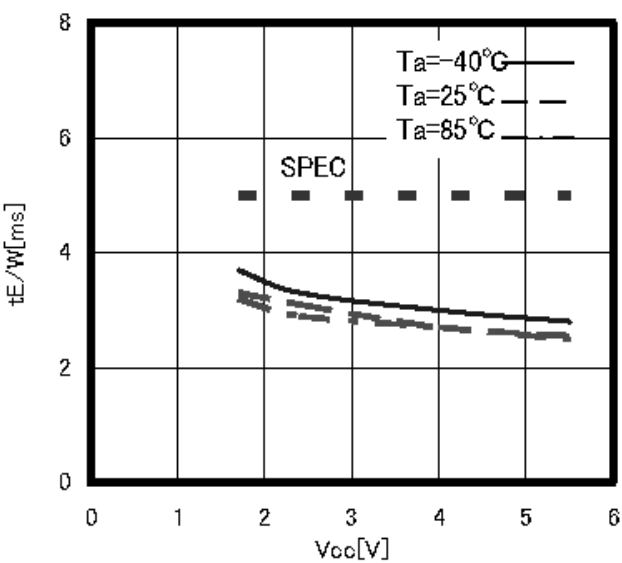
Figure 29. Write cycle time tE/W
