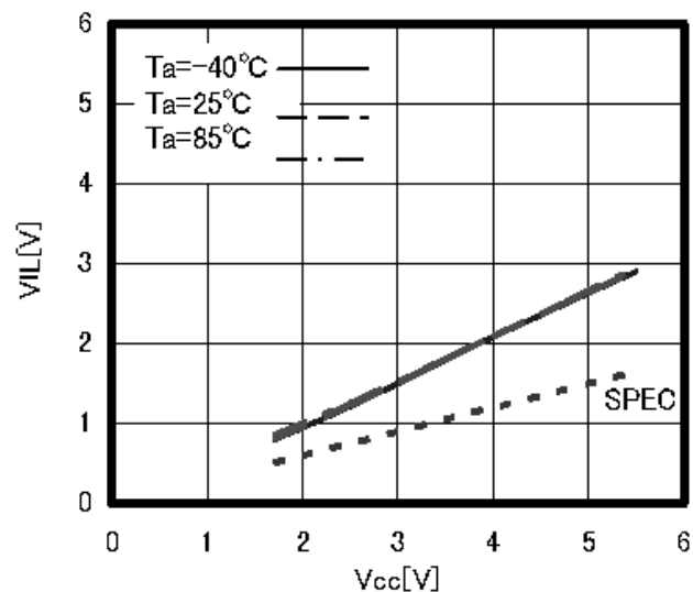
Figure 5. "L" Input Voltage V_{IL} (CSB, SCK, SI, HOLDB, \overline{\text{WP}} )
