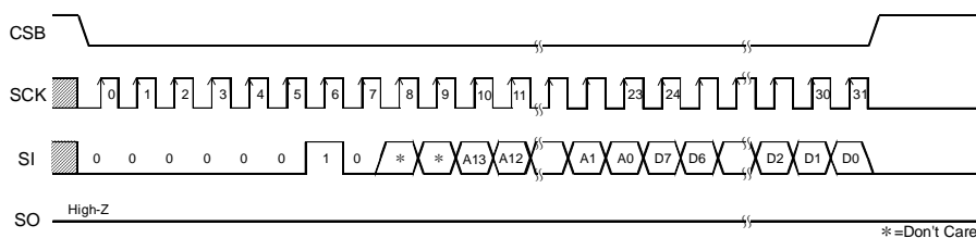
Figure 38. Write command
