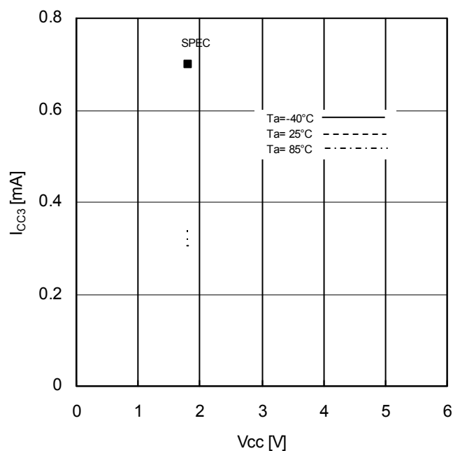
Figure 15. Supply Current (Read) vs Supply Voltage ( f_{SCK}=3\text{MHz} )
