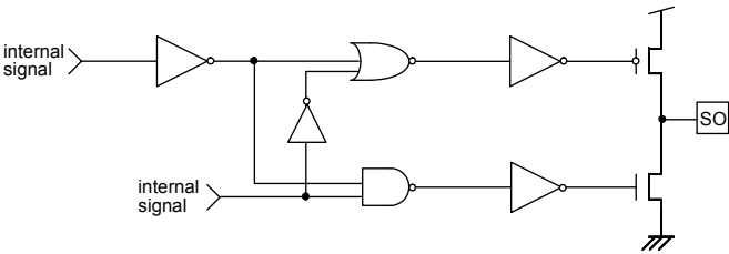
Figure 51. SO output equivalent circuit
