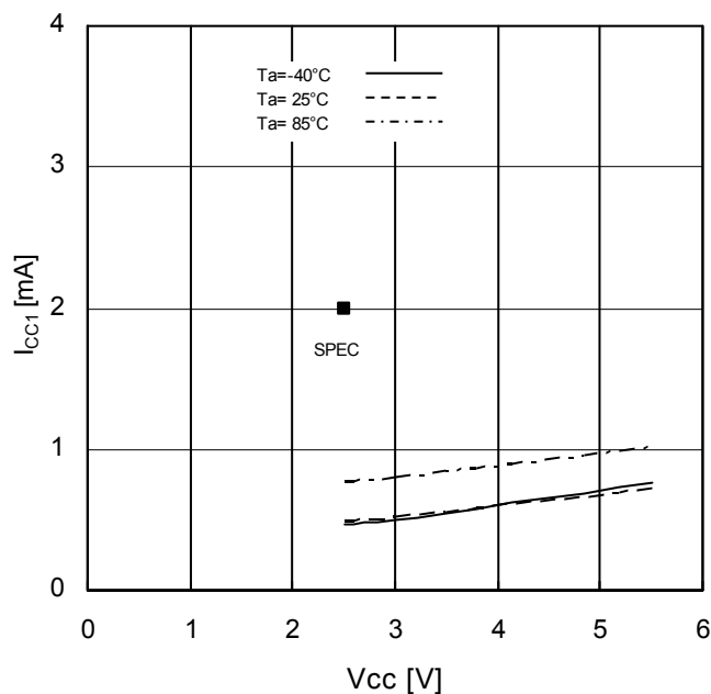
Figure 13. Supply Current (Write) vs Supply Voltage ( f_{SCK}=5\text{MHz} )
