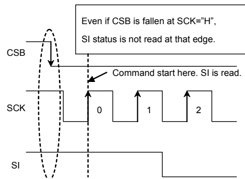
Figure 58. Operating timing
