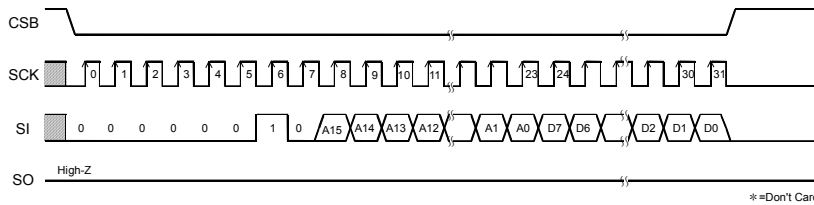
Figure 39. Write command
