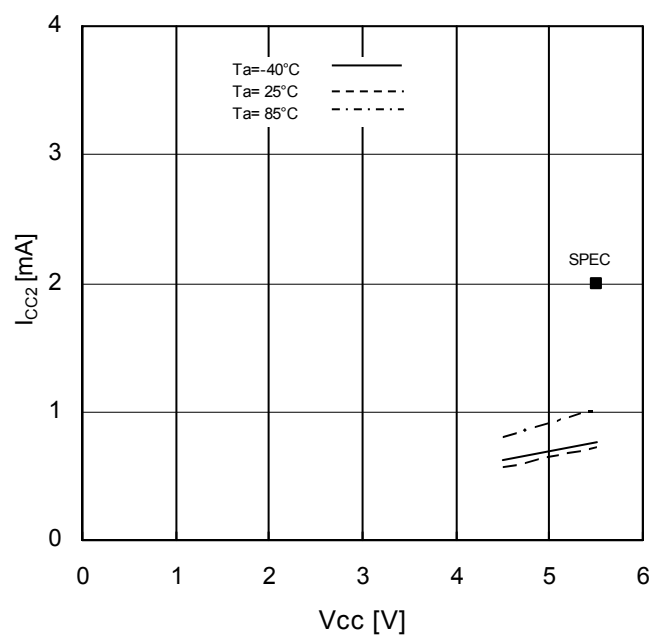
Figure 14. Supply Current (Write) vs Supply Voltage ( f_{SCK}=10\text{MHz} )
