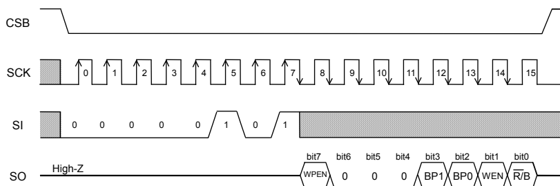
Figure 41. Read status register command
