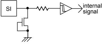
Figure 54. SI input equivalent circuit
