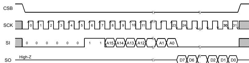
Figure 38. Read command
