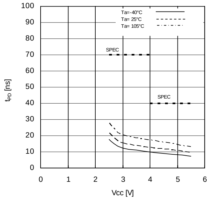
Figure 22. Data Output Delay Time vs Supply Voltage
