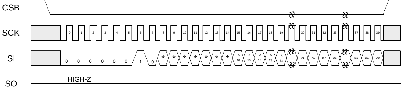
Figure 34. Write command
