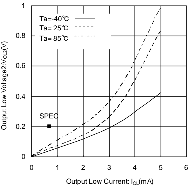
Fig 7. Output Low Voltage2 vs Output Low Current ( V_{CC}=1.6\text{V} )
