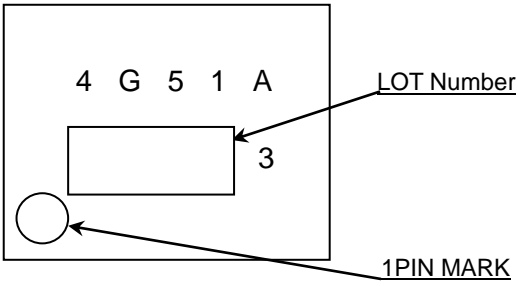
SOP8(TOP VIEW)
