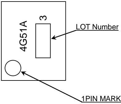
TSSOP-B8(TOP VIEW)
