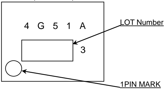
SOP-J8(TOP VIEW)
