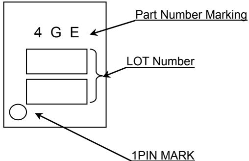
SSOP-B8(TOP VIEW)
