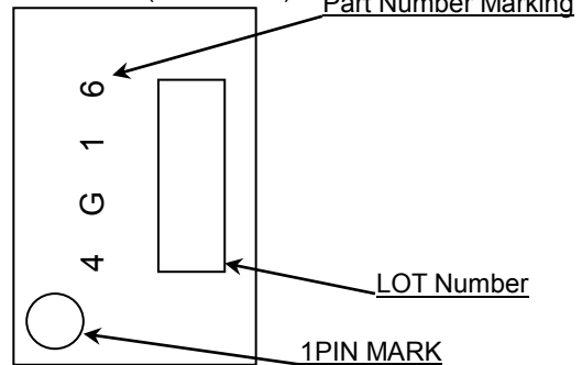
TSSOP-B8(TOP VIEW)
