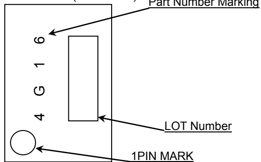
TSSOP-B8M(TOP VIEW)
