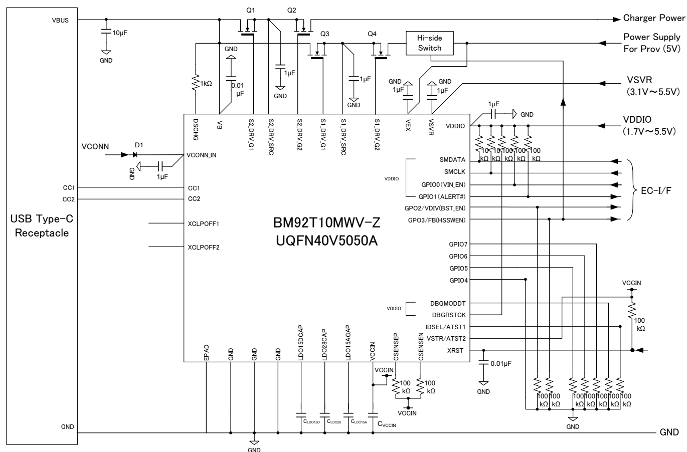
Figure 5-1 Application Example
