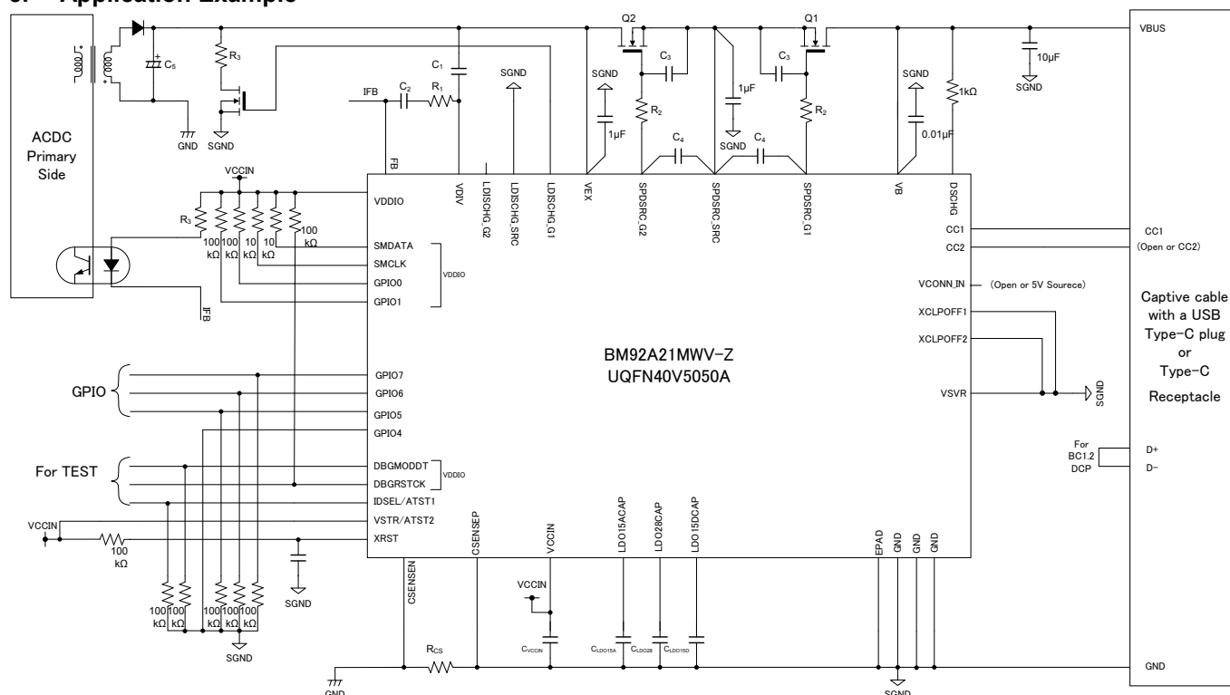
Figure 5-1 Application Example
