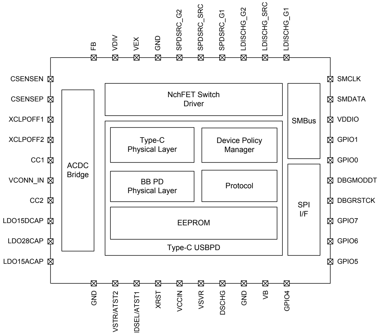
Figure 3-1 Block Diagram
