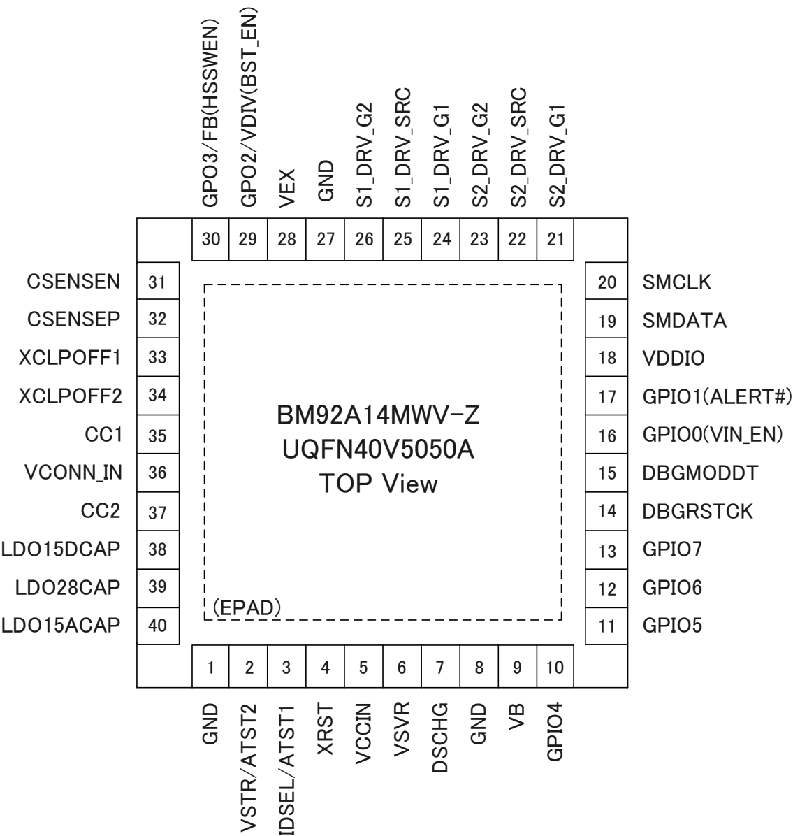
Figure 1-1 Pin configuration
