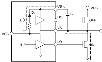
Figure 10. Charging Period
