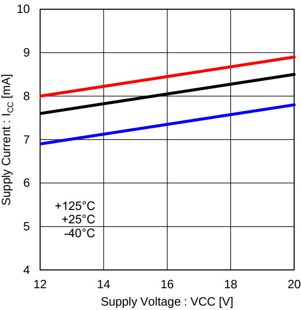
Figure 15. Low Side Drivers Operating Current ( f_{PWM} : 20kHz)
