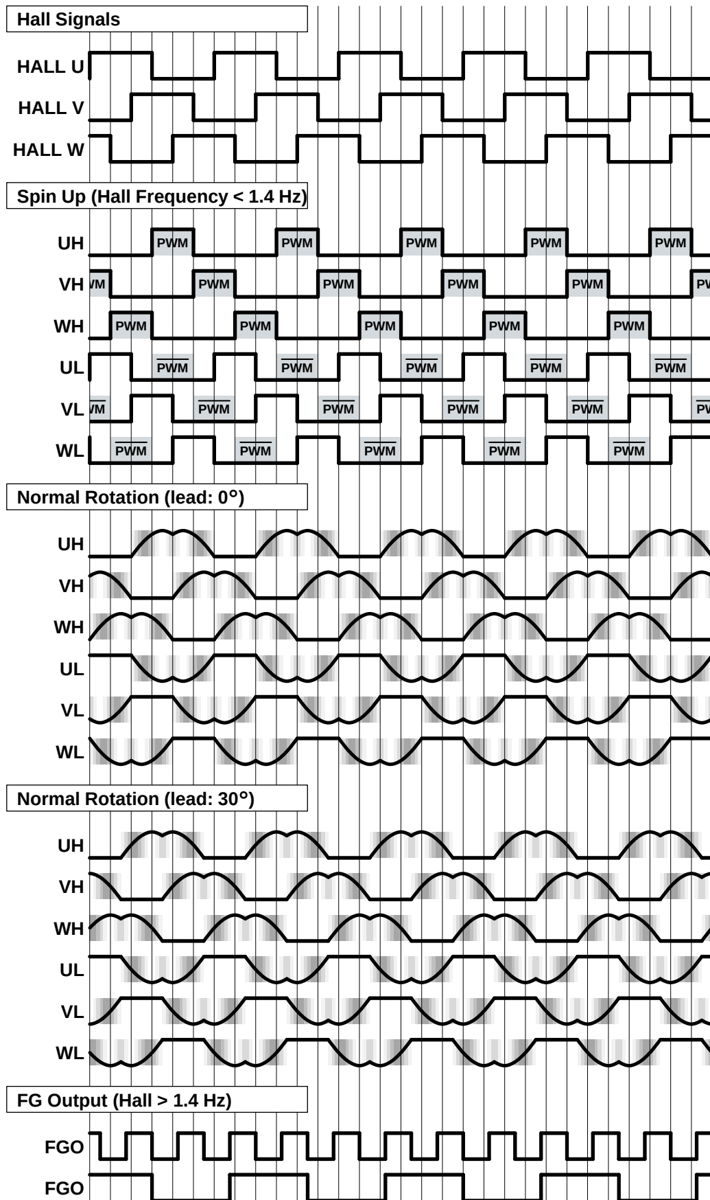
Figure 46. Timing Chart (Clockwise)
