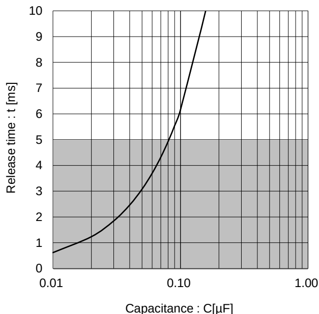
Figure 9. Release Time (Reference Data @R=100k \Omega )
