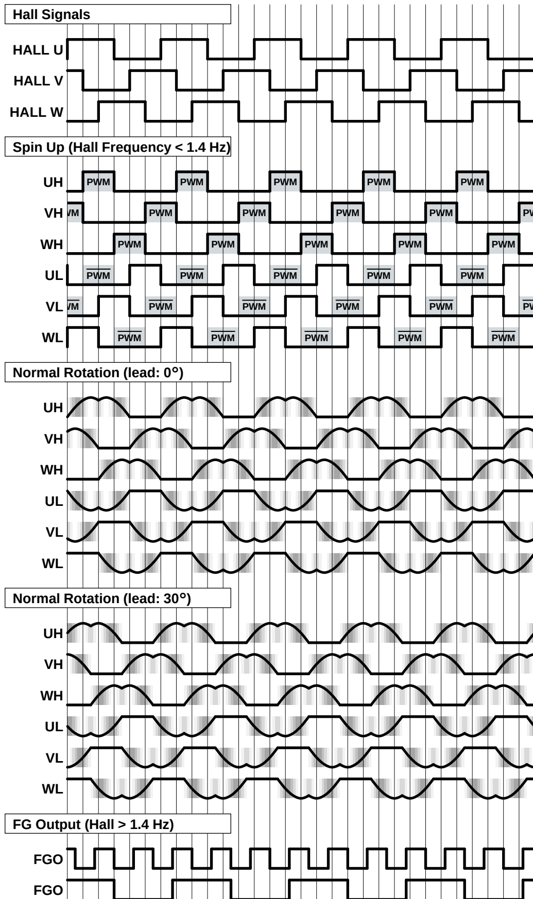
Figure 47. Timing Chart (Counter Clockwise)
