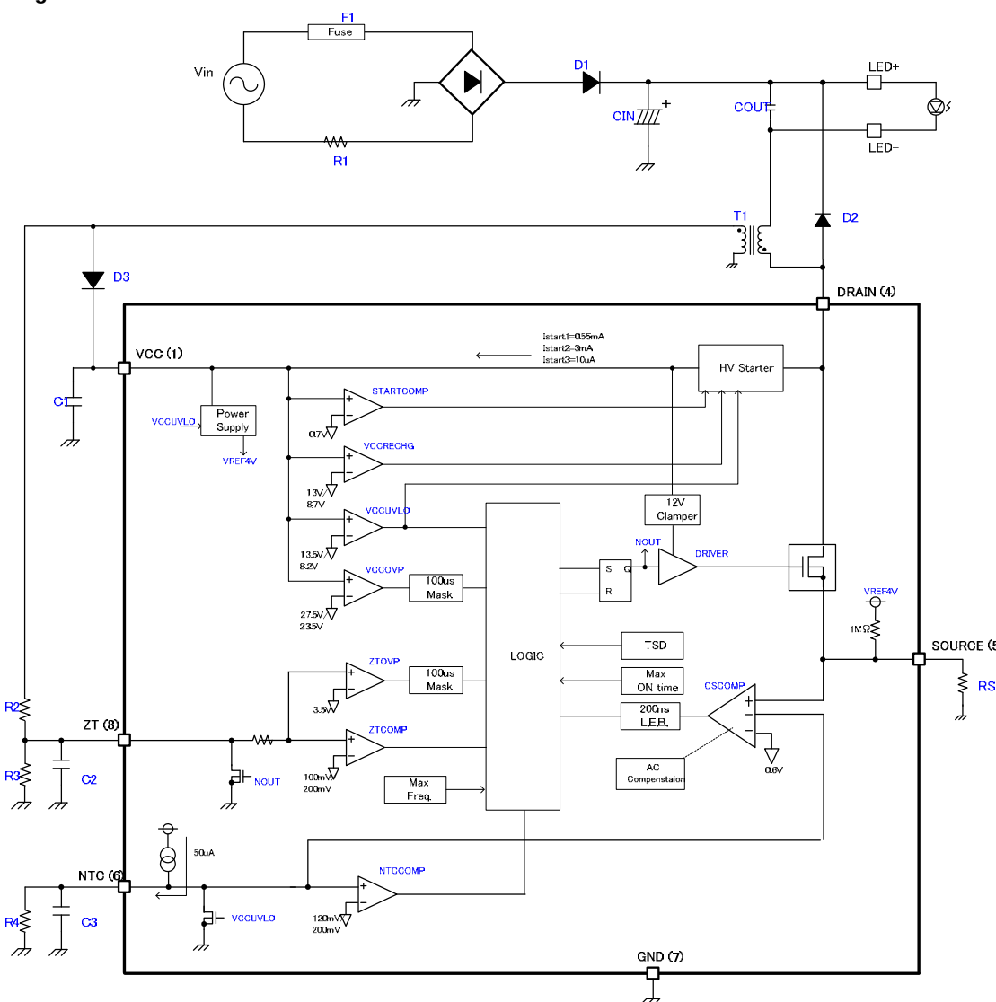
Figure 3. Block diagram
