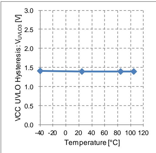
Figure 23. VCC UVLO Hysteresis vs Temperature (BM2P131X-Z, BM2P141X-Z, BM2P151X-Z, BM2P161X-Z, BM2P181X-Z, BM2P201X-Z, BM2P241X-Z)
