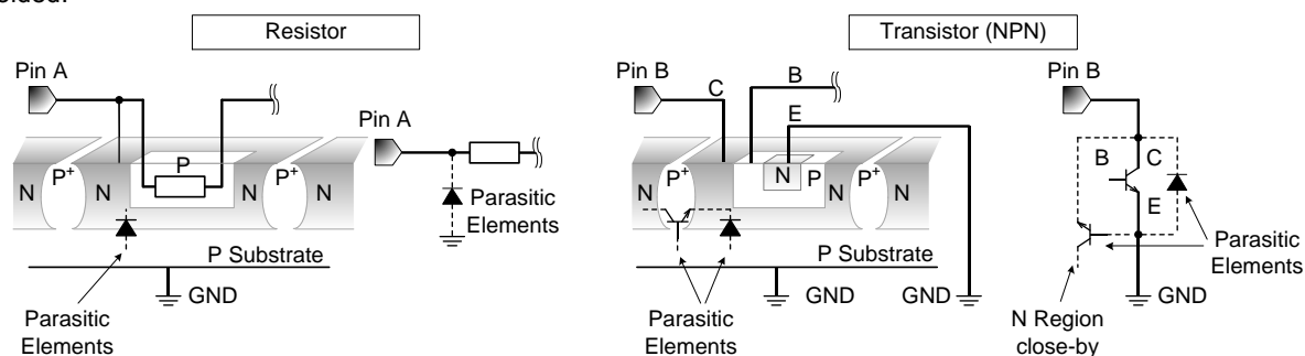
Figure 35. Example of IC Structure
