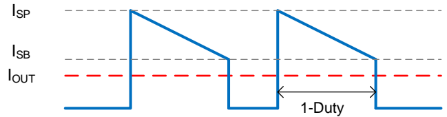
Figure 7. Secondary Current
