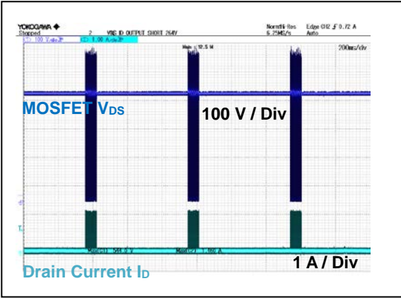
Figure 26. Diode Wave Form V_{IN} = 264 Vac Output Shorted
