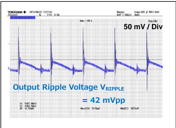
Figure 31. V_{IN} = 115 \text{ Vac} , I_{OUT} = 0.5 \text{ A}
