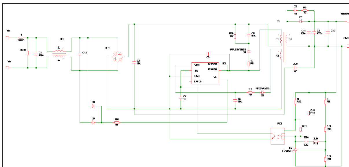
Figure 3. Application Circuit
