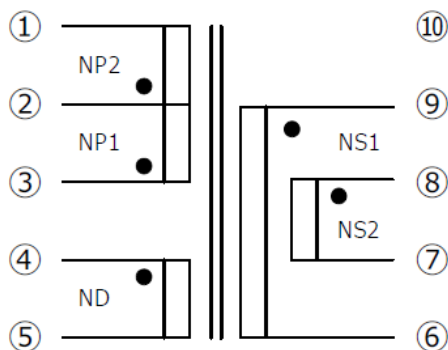
Figure 8. Circuit Diagram
