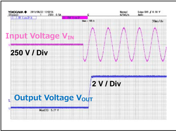
Figure 28. V_{IN} = 264 Vac, I_{OUT} = 0.5 A
