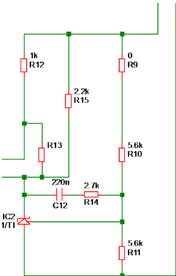
Figure 13. Feedback Circuit
