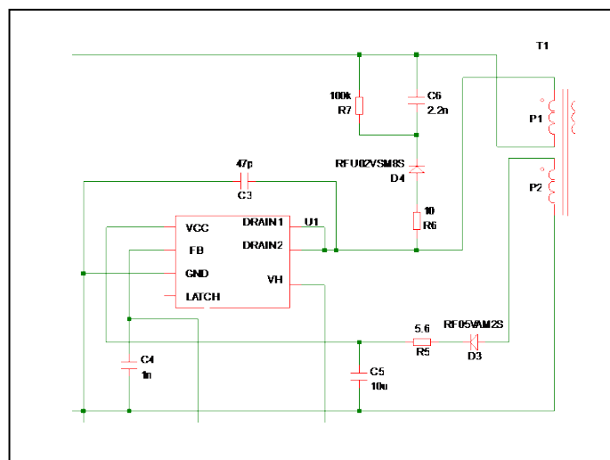
Figure 8. Circuit around BM2P26CK-Z
