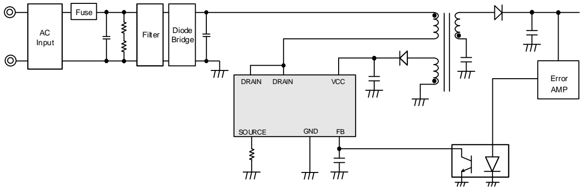
Figure 33. Flyback Application Ciucit
