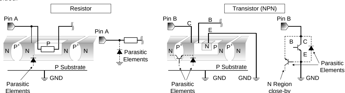
Figure 37. Example of IC Structure
