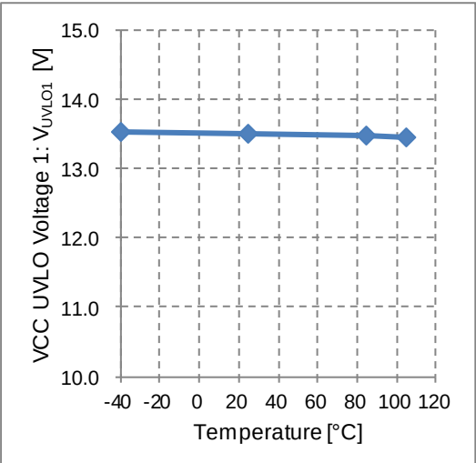
Figure 16. VCC UVLO Voltage 1 vs Temperature
