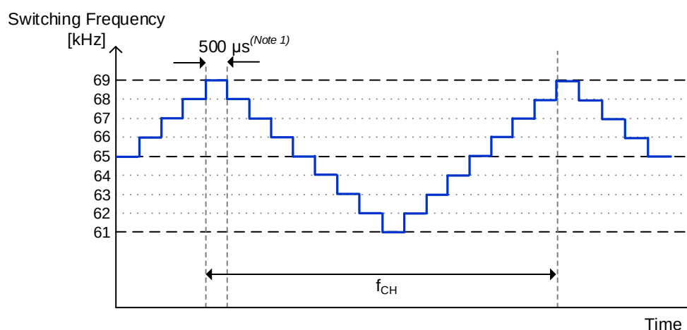
Figure 5. Frequency Hopping Function
