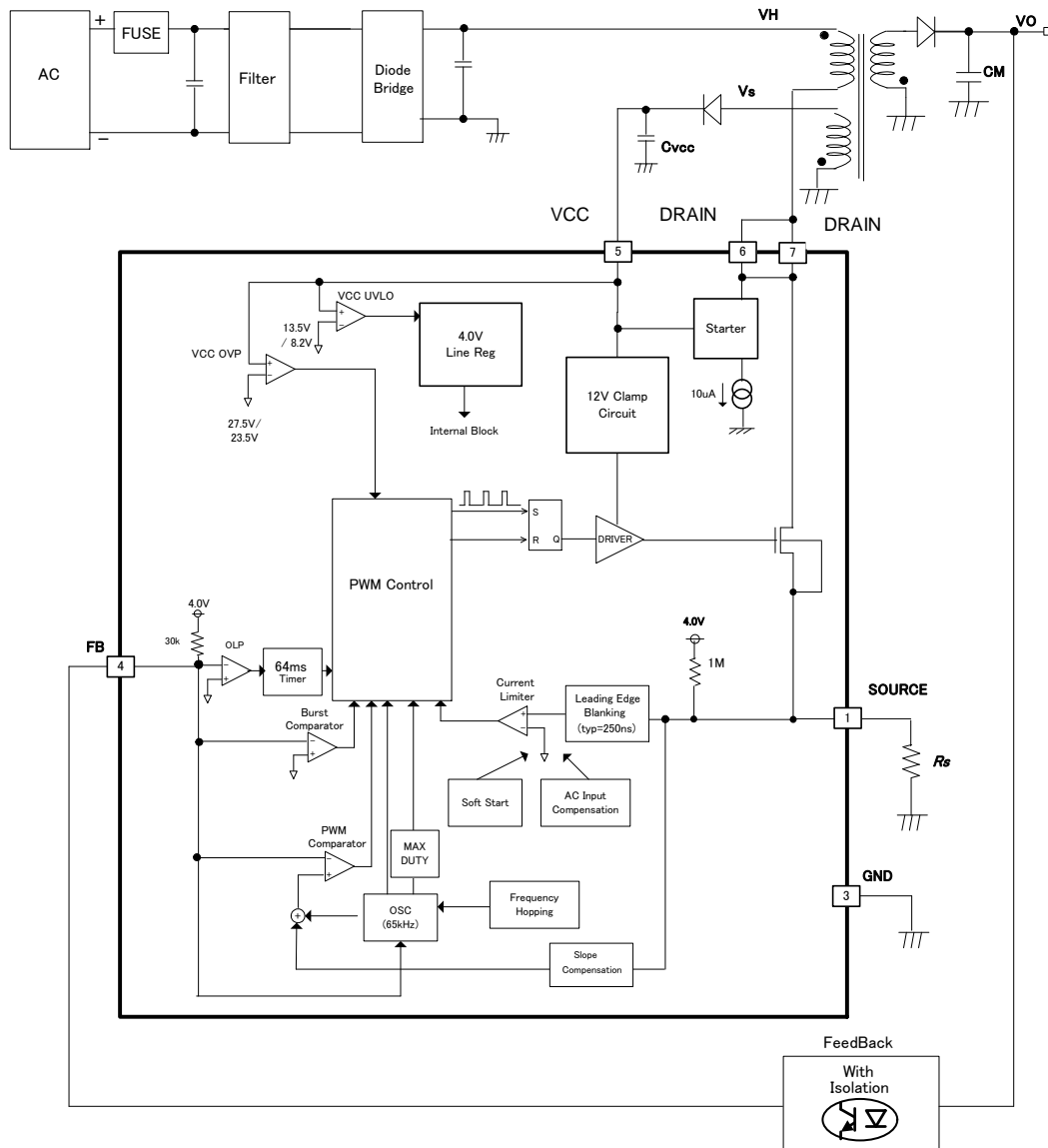
Figure 3. Block Diagram
