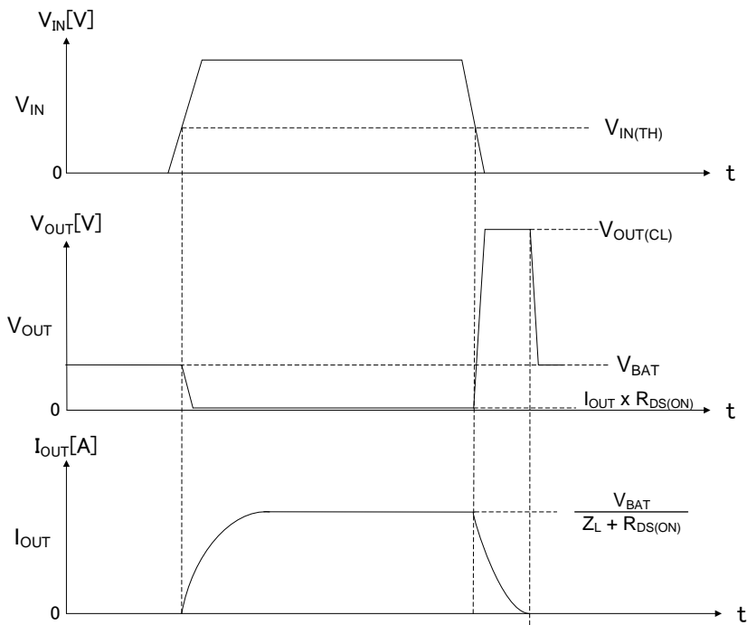
Figure 34. Inductive Load Operation
