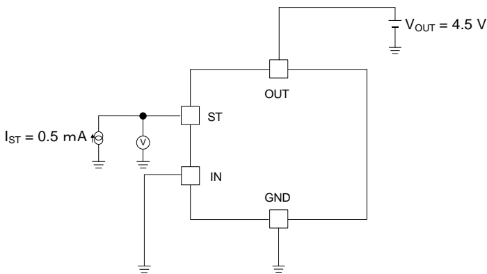
Measurement Circuit for Figure 28
