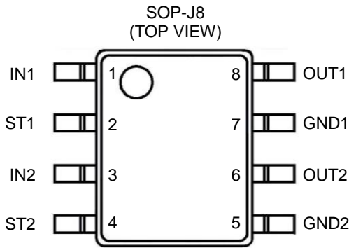
Figure 2. Pin Configuration
