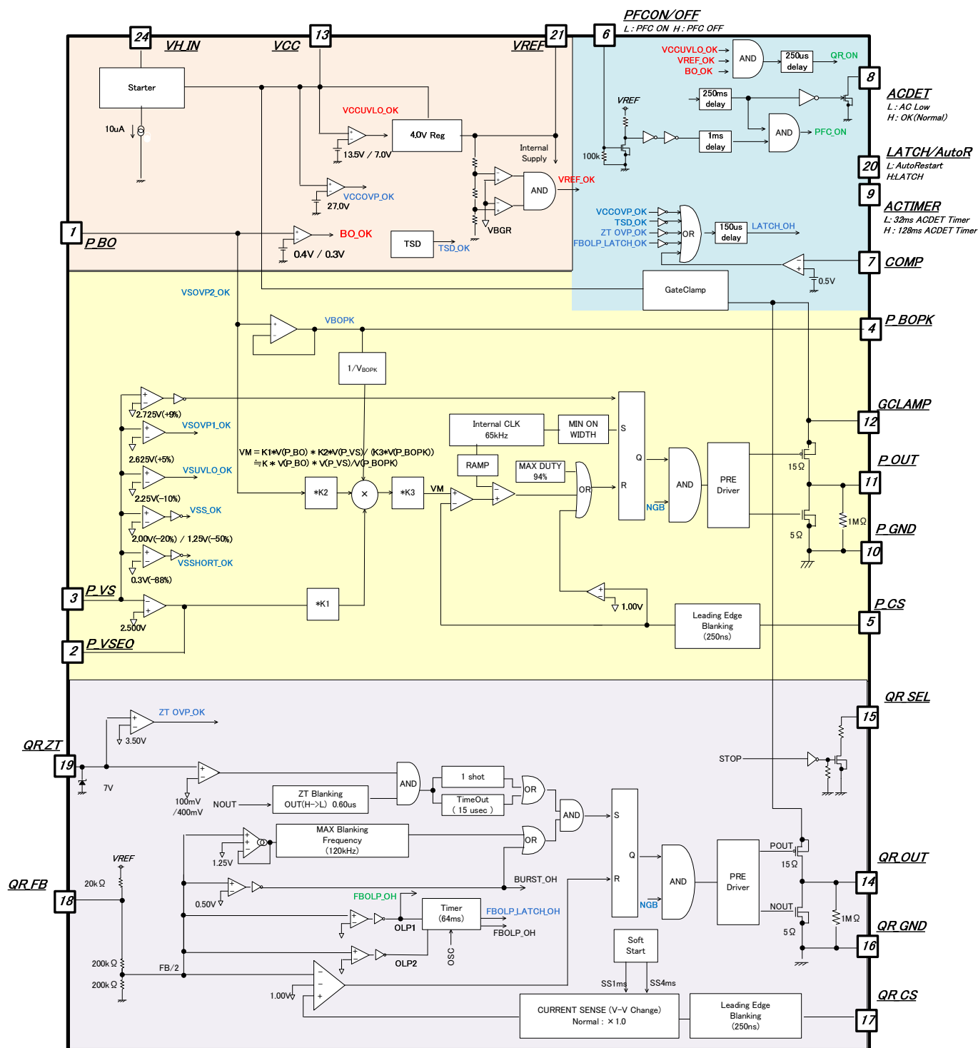
Figure 3-2. Block Diagram
