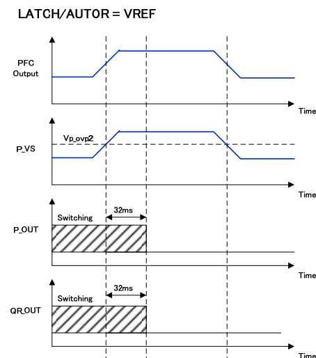
Figure 45. Operation of P_VS Second Over Voltage Protection (at latch mode)
