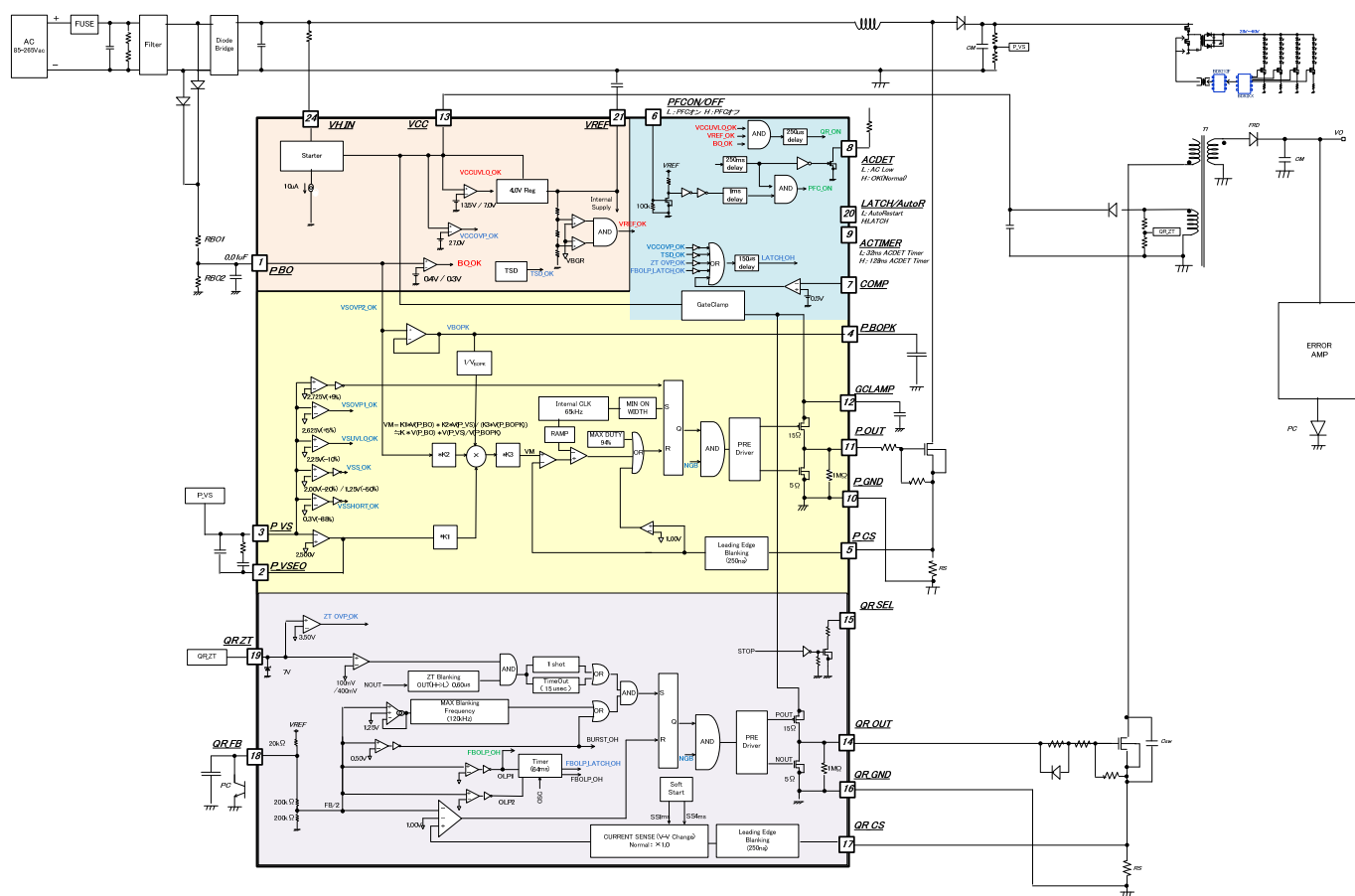
Figure 3. Block Diagram
