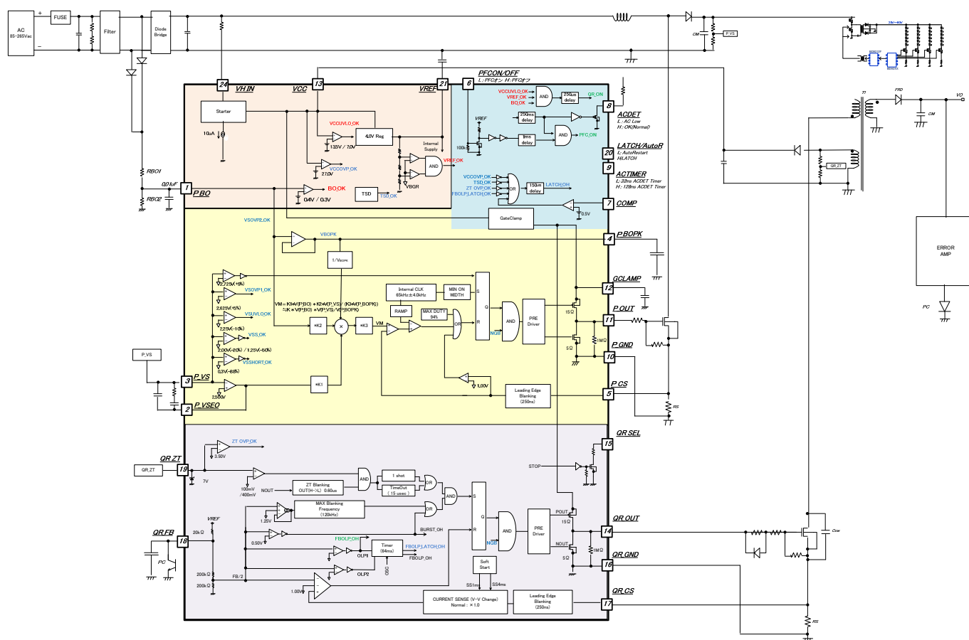
Figure 3. Block Diagram
