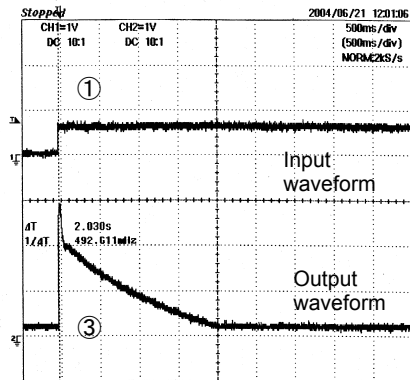
Fig10 Relationship of Output Voltage to Input Voltage (For BH76106HFV C_{in}=1\mu\text{F} )
