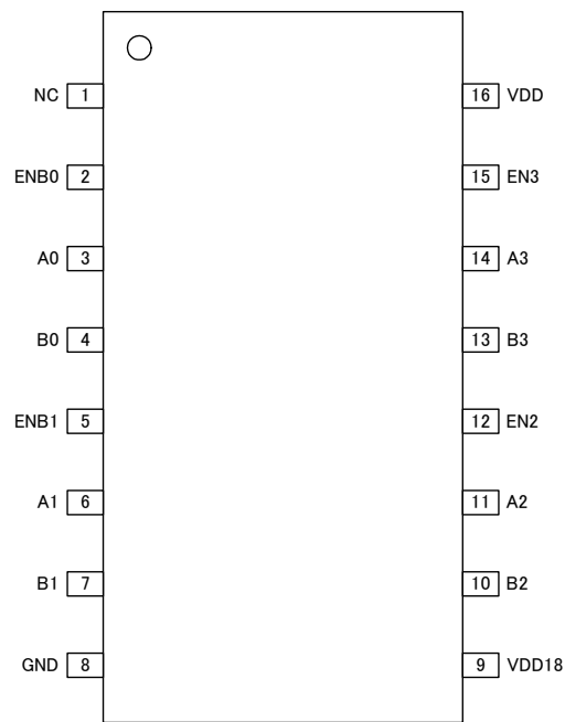
Fig.7 Pin configuration
