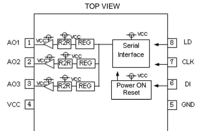
Figure 2. BH2220FVM
