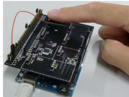
Figure 6. Measurement Environment
