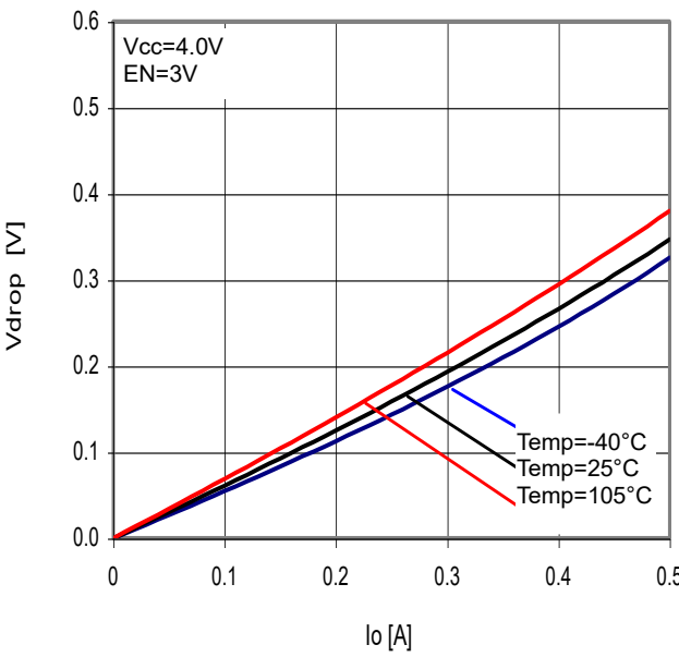
Fig.36 Minimum dropout Voltage 3 (VCC=4.0V)
