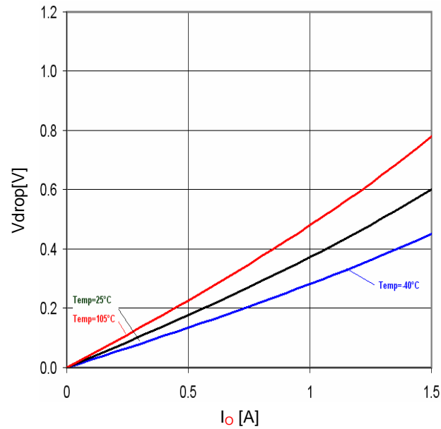
Fig.34 Minimum dropout Voltage 2 ( V_{CC} =4.5V、 T_a =25°C)
