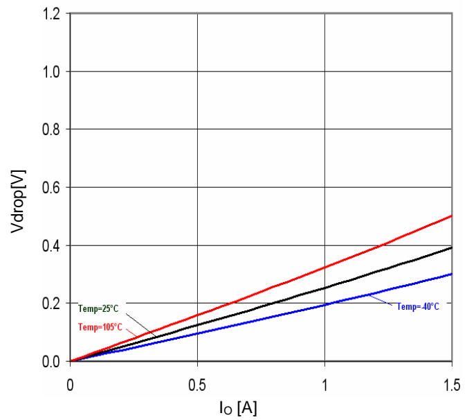
Fig.36 Minimum dropout Voltage 2 (V CC =8V, Ta=25°C)
