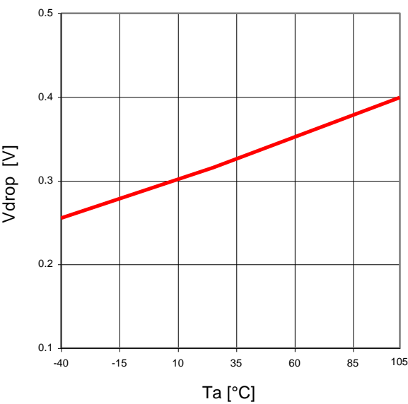
Fig.33 Ta-Vdrop (Vcc=6V, Io=0.3A)
