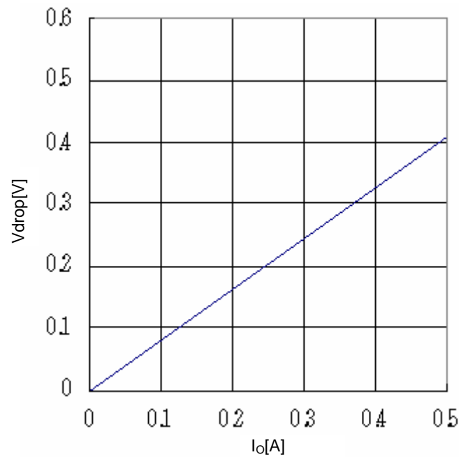
Fig.22 Minimum dropout Voltage 2 ( V_{CC}=4.5\text{V} , T_a=25^\circ\text{C} )
