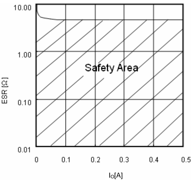
Fig.19 ESR condencer
